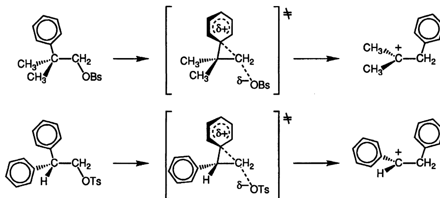
Scheme 1. Solvolytic processes of neophyl and 2,2-diphenylethyl systems.
