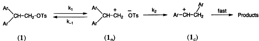
Scheme 3. Pre-equilibrium mechanism.
